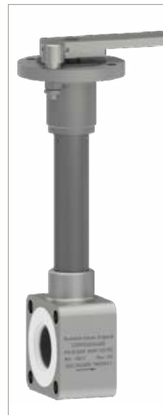
Centre-Section for Parker Bestobell Cryogenic Ball Valves
