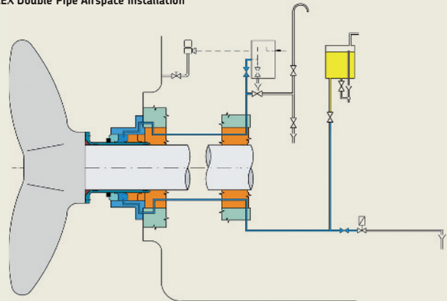
SIMPLEX Double Pipe Airspace installation
