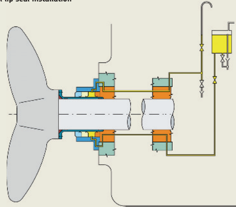
Typical lip seal installation
